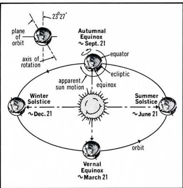
Figure I-2. Path of ecliptic traced by position of sun as earth moves about it.
