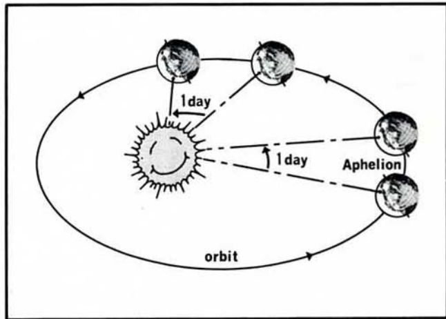
Figure I-1. Presentation of earth's orbital motion exaggerated to show varying effects on apparent solar day.
