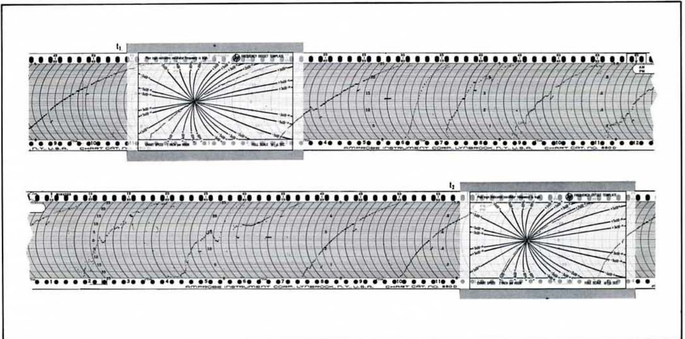
Figure 2-9. Use of template to interpret 117A recording
