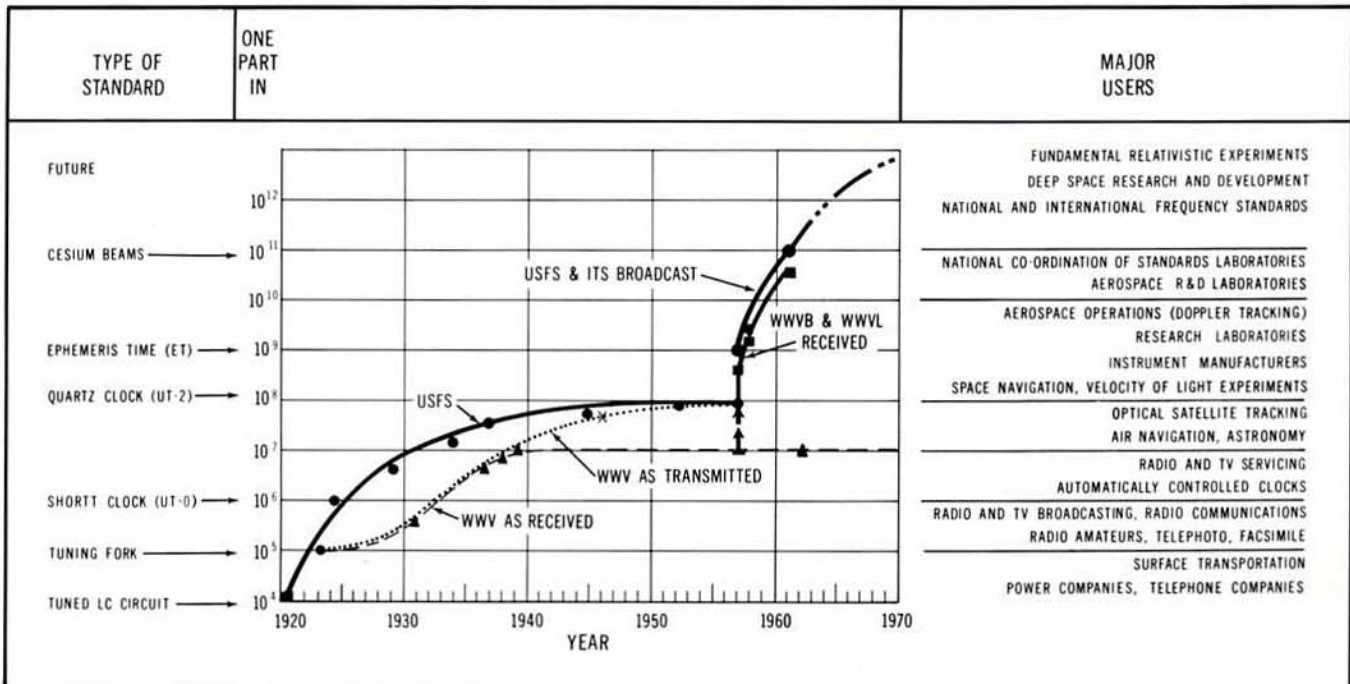
Figure II-1. Improvements in the precision of the U.S. Frequency Standard (USFS) and its dissemination.
