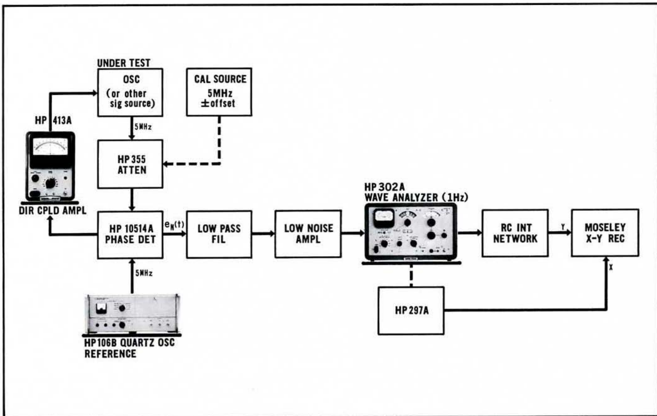
Figure 3-5. Instrumentation setup for plotting phase noise versus frequency offset
