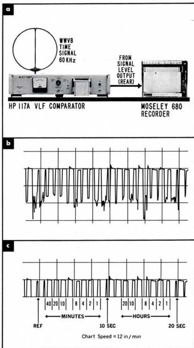
Figure 2-13. Equipment to produce a time record (a), a trace (less than a minute) produced with this equipment (b), and the same trace with a template superimposed to aid in its interpretation (c).
