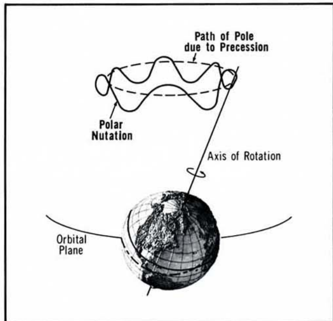
Figure I-6. Nutation superimposes a seasonal wavy motion on the circular path of precession.
