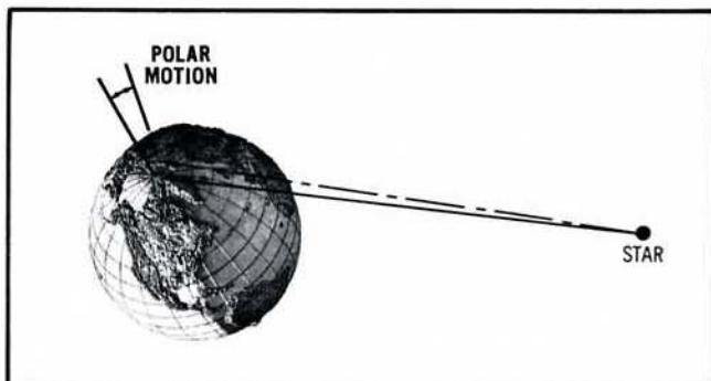
Figure I-3. Polar motion changes the apparent position of a fixed point of observation with respect to a distant celestial body.
