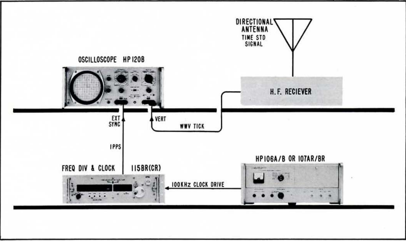
Figure 2-1. Equipment for time comparison with tick phasing adjustment
