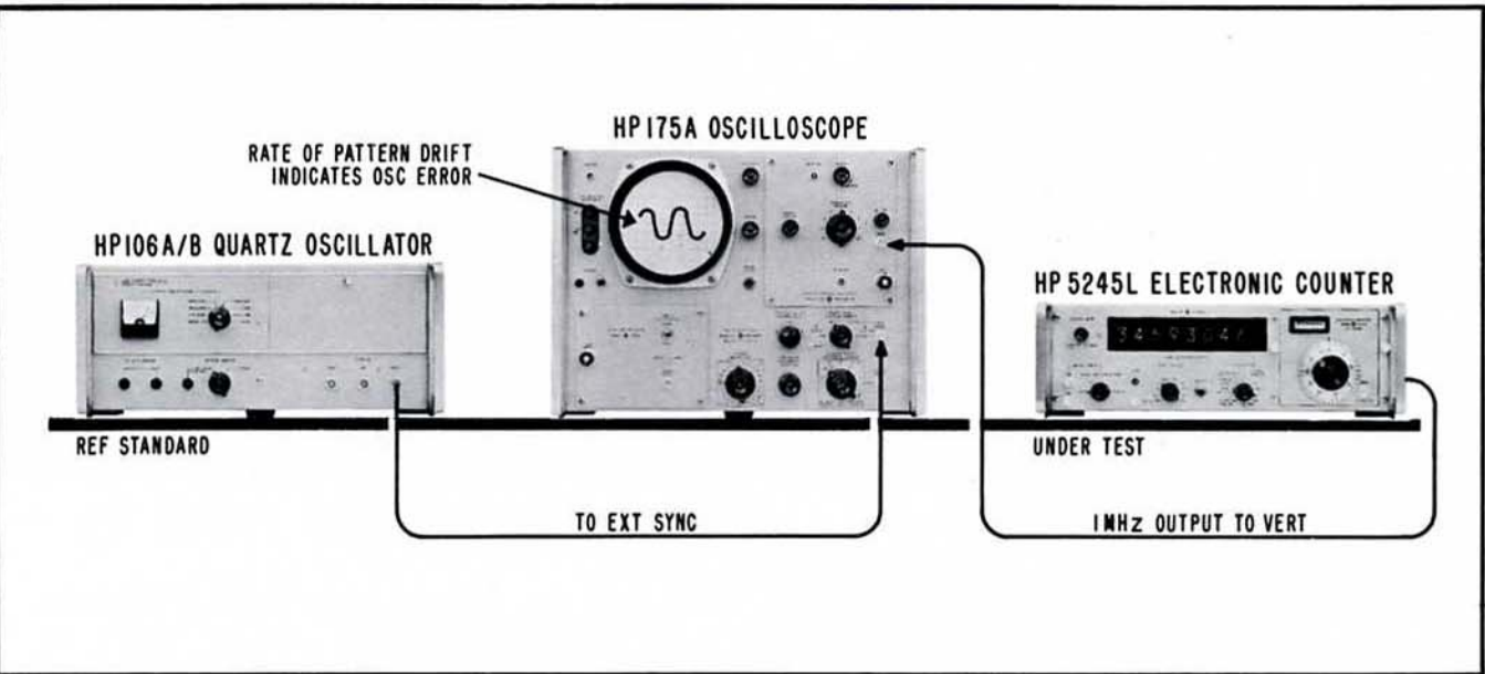
Figure 3-2. Equipment to check a counter's internal oscillator.
