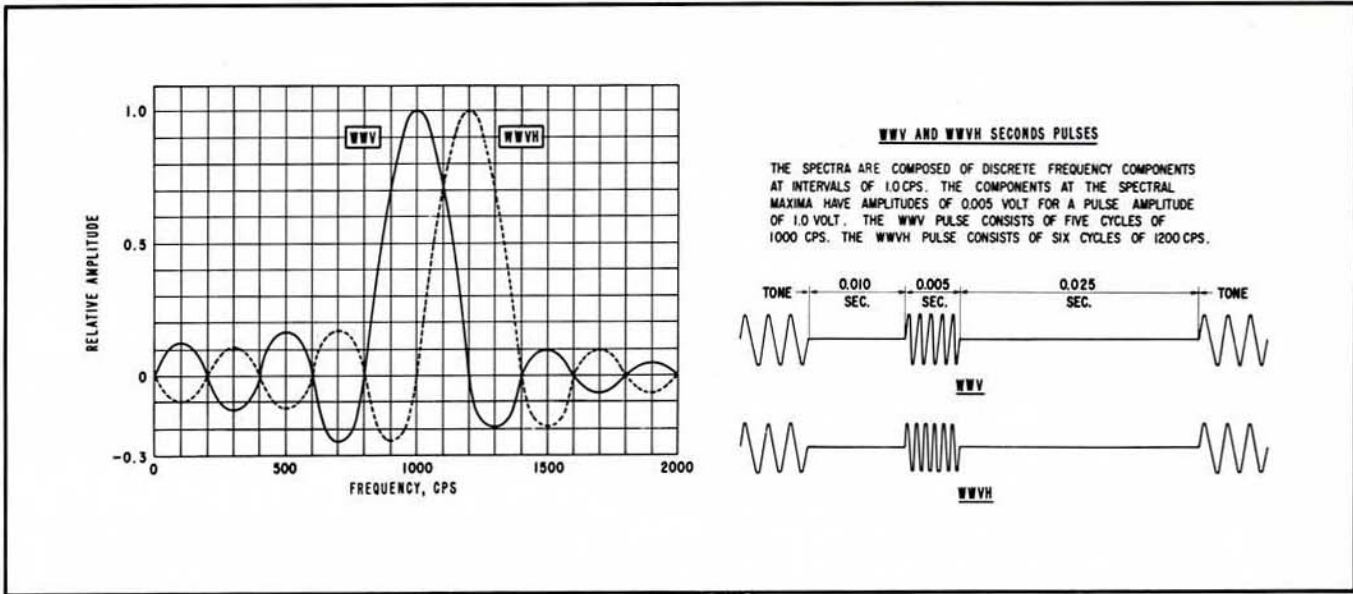
Figure III-2. Sample Characteristics of Time Pulses Broadcast from NBS Stations WWV and WWVH.
