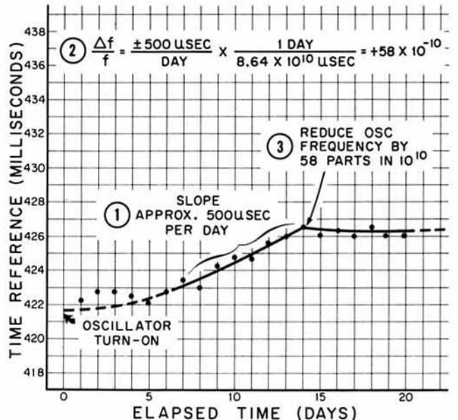
Figure 4-9. Time Comparison Plot
