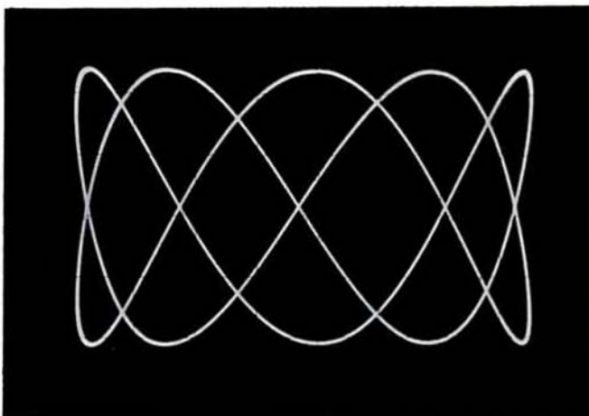
Figure 3-1. Lissajous pattern (frequency ratio 5:2).
