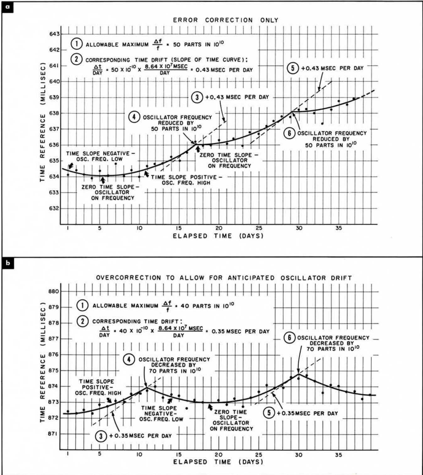
Figure 4-10. Slope-Limit Frequency Control
