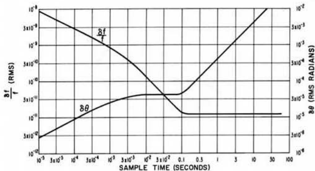
Figure 5-3. Maximum RMS fractional frequency deviation and maximum RMS phase deviation as a function of Sample Time for 5 MHz output of Model 106A,B Quartz Oscillators
