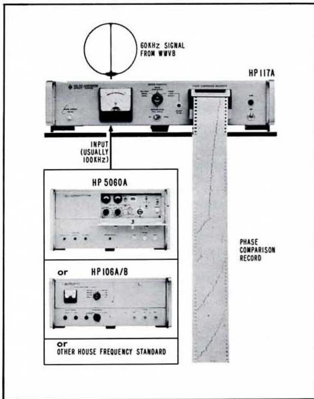
Figure 2-8. VLF Phase Comparison System
