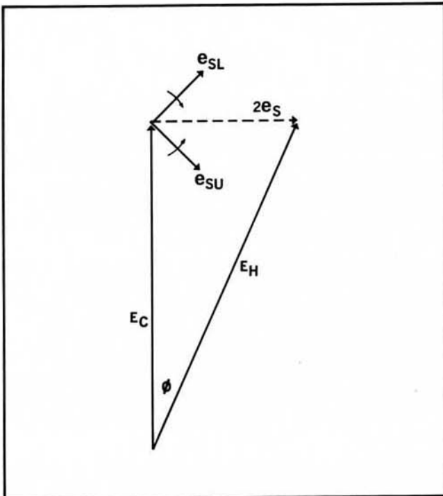
Figure 3-4. Vector representation of phase noise modulation
