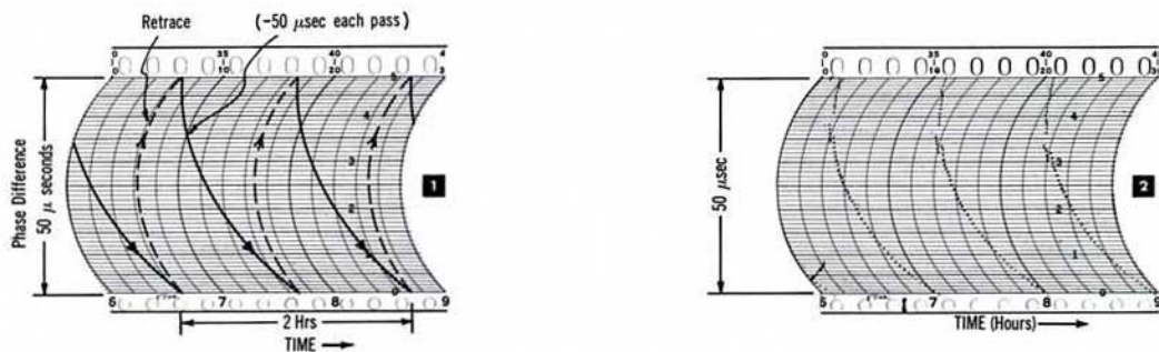
Figure 2-10 (c). Parts 1 and 2. Comparison Plots, UT 2 Local Standard without use of Translator
