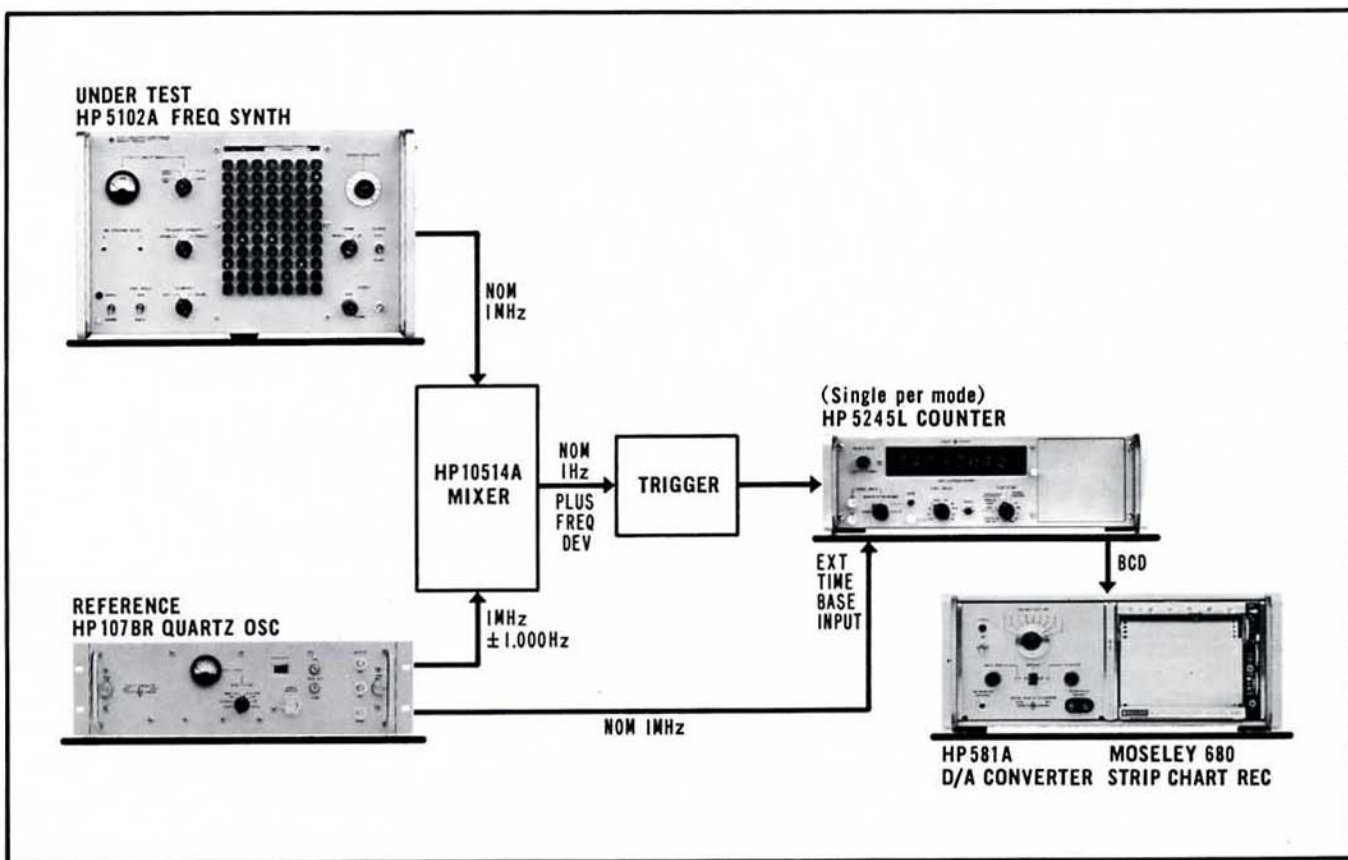
Figure 3-3. Block diagram for frequency comparison measurements.
