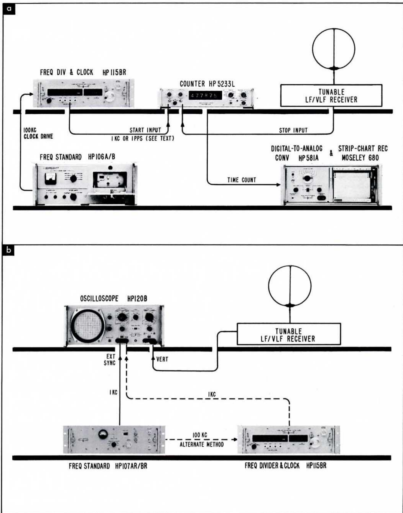
Figure 2-12. LF/VLF Comparison Systems
