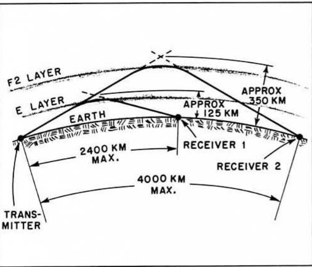
Figure 4-3. Single-hop sky-wave paths
