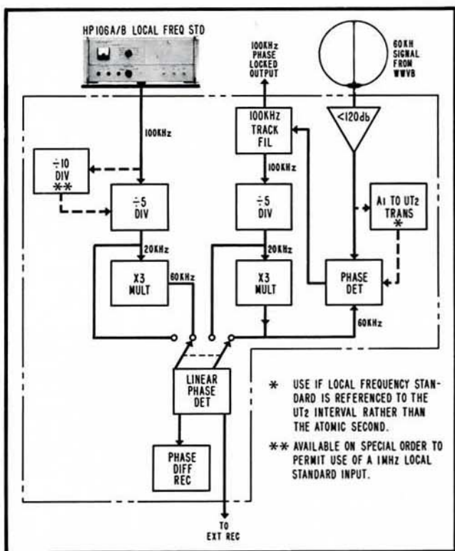
Figure 2-6. Simplified Diagram of the HP Model 117A VLF Comparator System
