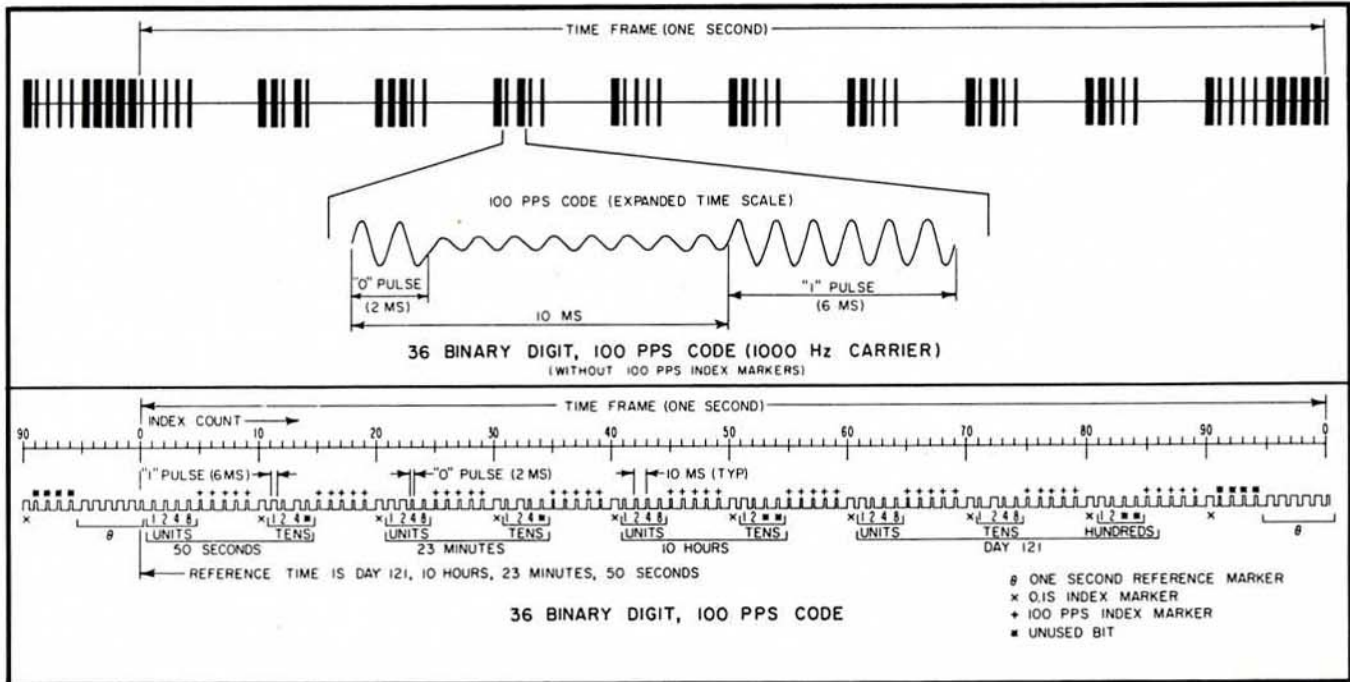
Figure III-3. Chart of Time Code Transmissions from NBS Station WWV.
