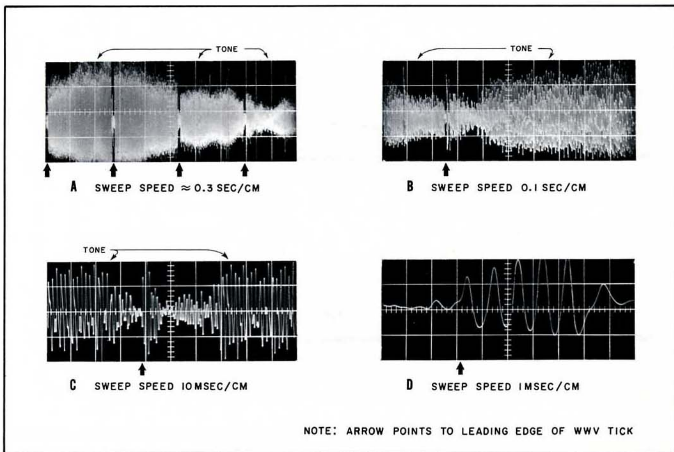
Figure 2-2. Typical oscillograms showing WWV signals
