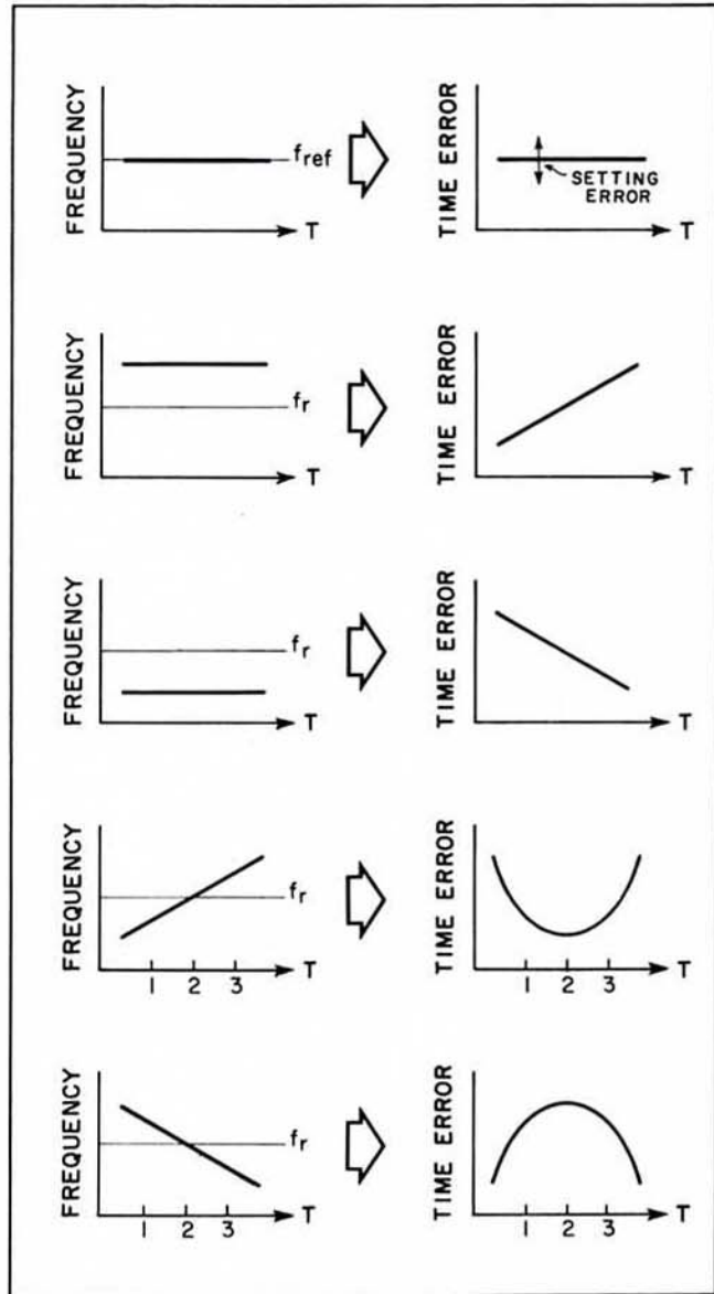
Figure 4-5. Corresponding frequency and time plots
