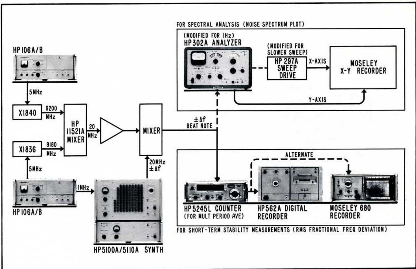
Figure 5-2. Versatile system for evaluating stability of quartz crystal oscillators
