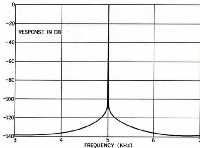
Figure 5-4. Spectrum of a 5 kHz Beat Note at 9.2 GHz (106A/B vs 106A/B)
