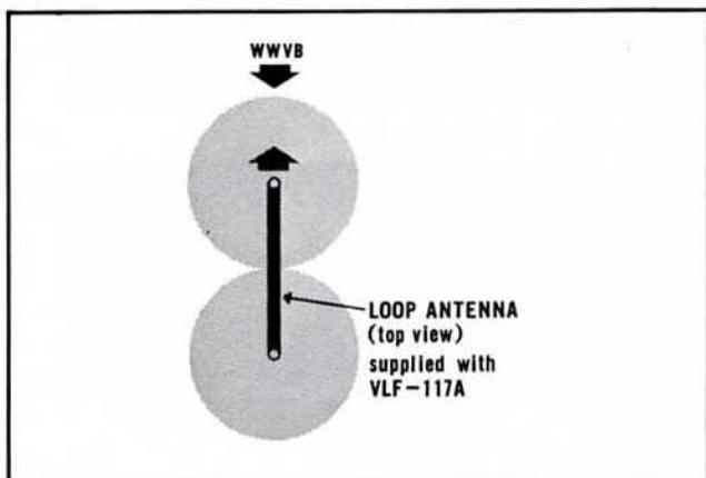
Figure 2-7. Orientation of VLF-117 Antenna for maximum signal pick-up
