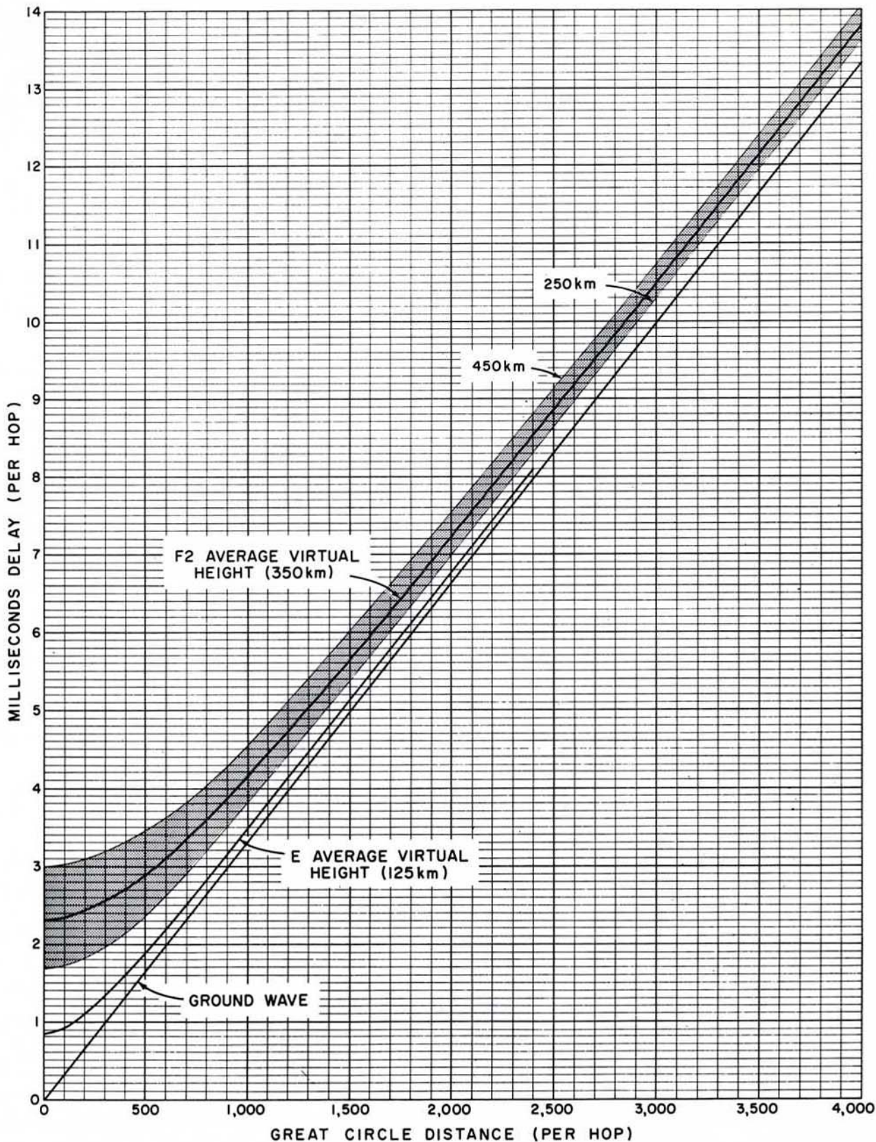
Figure 4-2. Transmission Delay Graph
