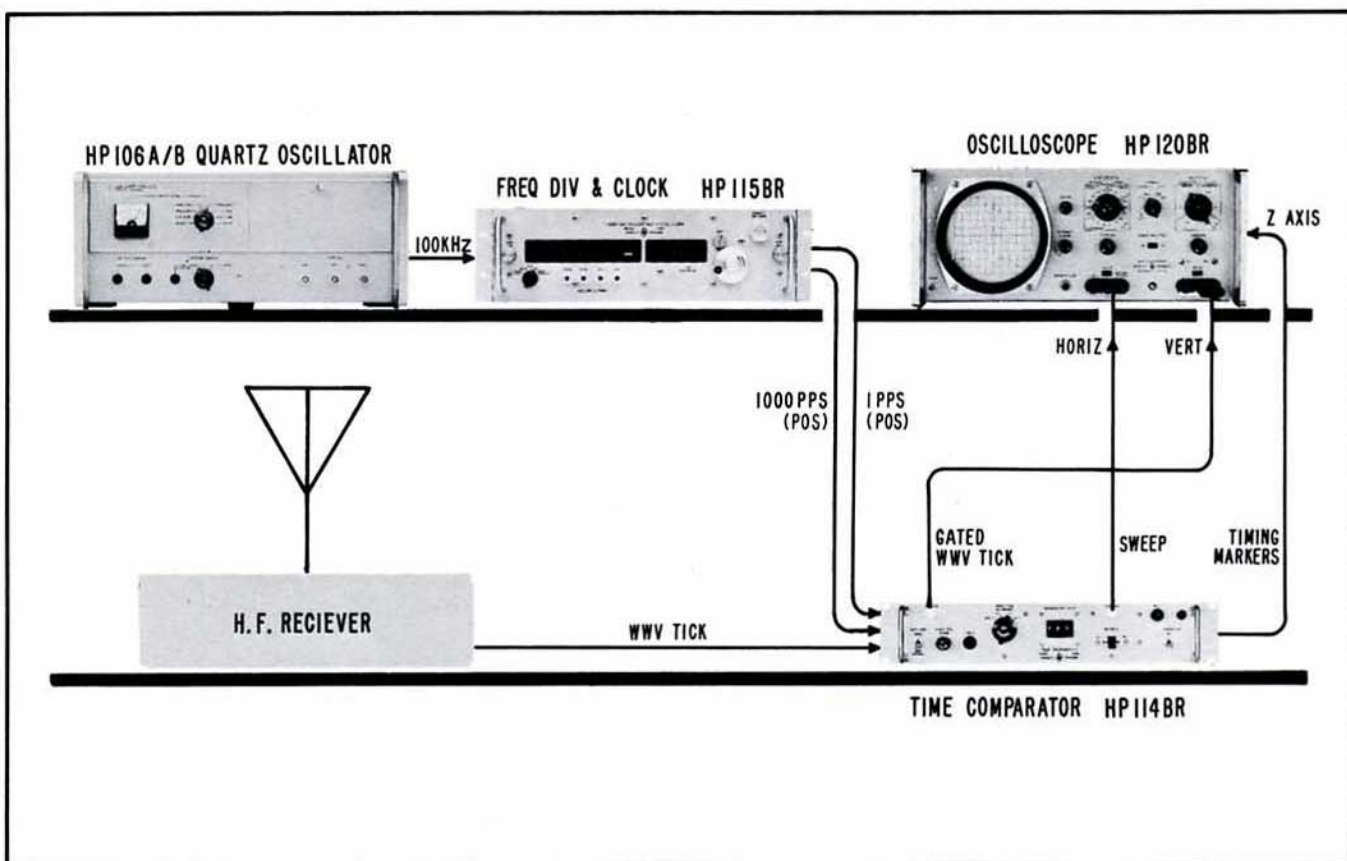
Figure 2-3. Equipment for time comparison simplified by use of HP-114BR Time Comparator
