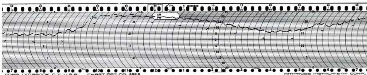
b Phase comparison plot, HP house standard vs WWVB, 16\frac{2}{3} \mu s full scale, Mar 4, 1965
