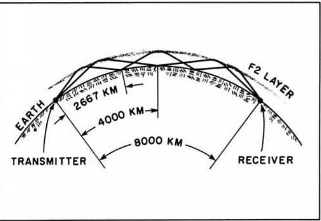
Figure 4-4. Multiple-hop transmission path
