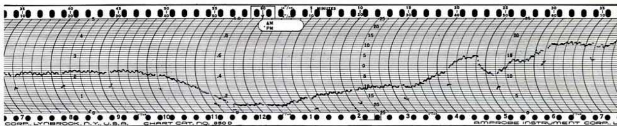
a Phase comparison plot, HP house standard vs WWVB, 16\frac{2}{3} \mu s full scale, Jan 21, 1965
