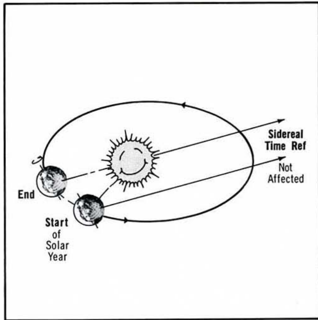
Figure I-5. Precession of the equinoxes causes the solar year to be about 20 minutes shorter than the sidereal year.
