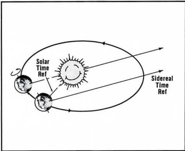
Figure I-4. Since the length of the solar day is referenced to the sun, orbital motion lengthens the solar day over what it would be if the earth were fixed in position. Sidereal time is referenced to distant stars; orbital motion is of no consequence.
